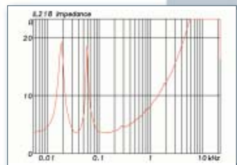
Impedance
